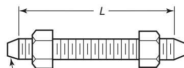
Point height [Note (1)] Stud Bolt With Nuts
